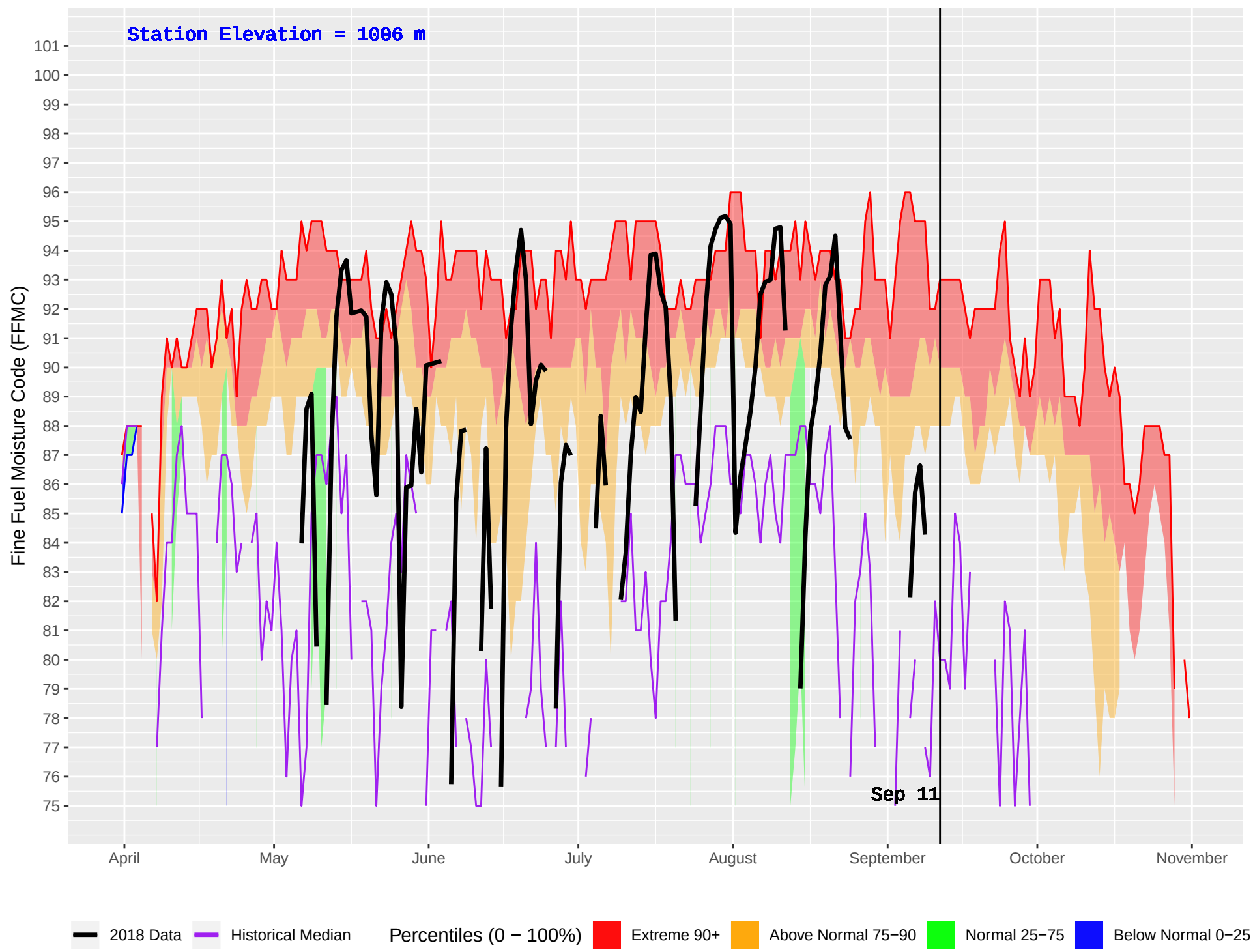
BENSON (228) : Historical (1987–2016) and Current (2018) Daily Fine Fuel Moisture Code (FFMC)
